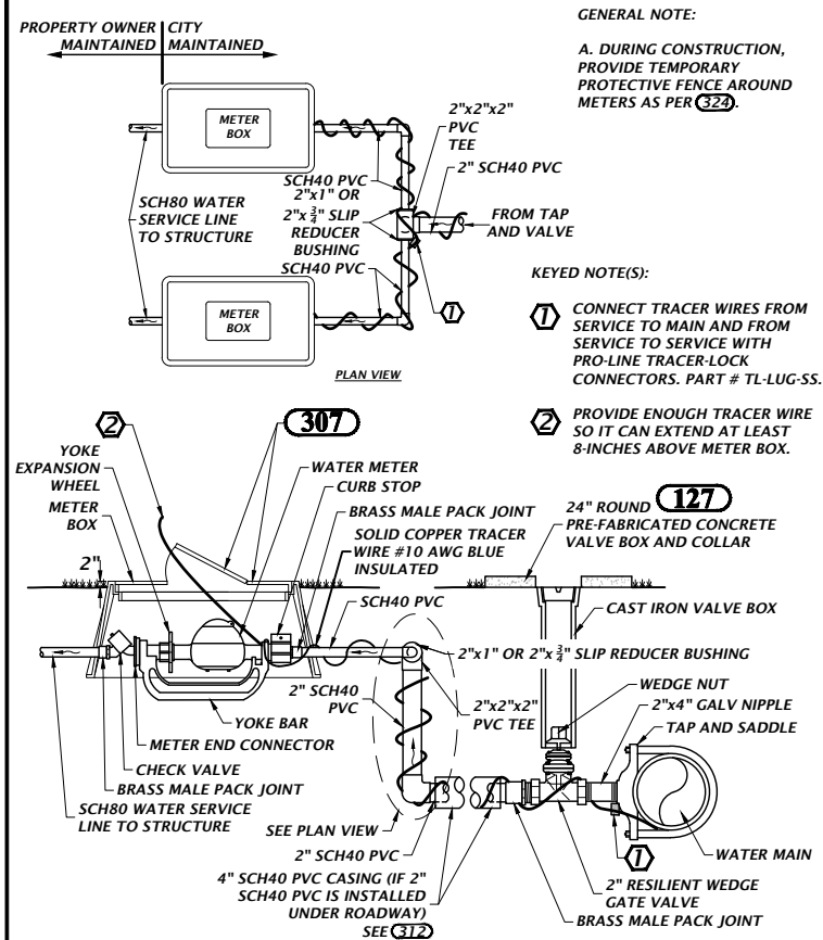
130 DUAL WATER SERVICE CONNECTION NTS
