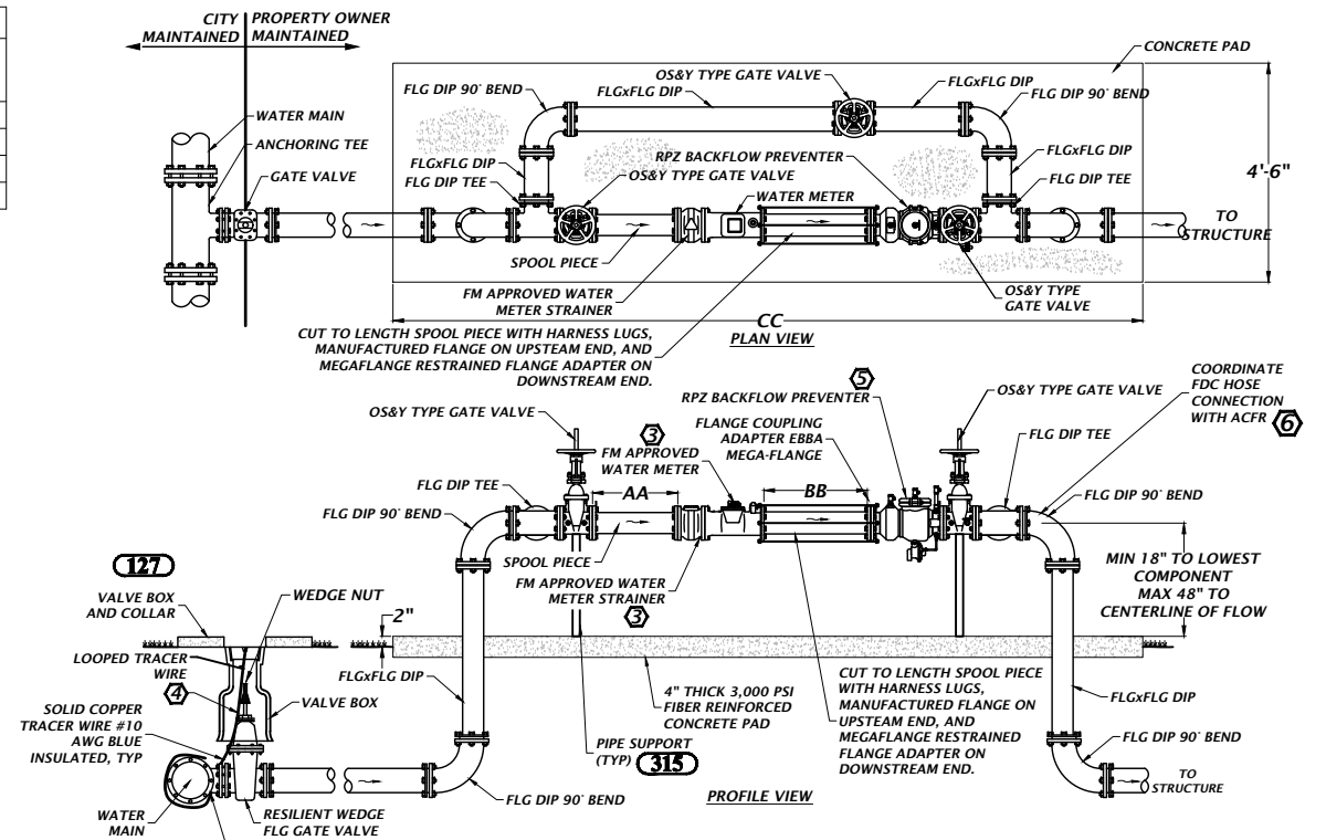
130 DUAL WATER SERVICE CONNECTION NTS
