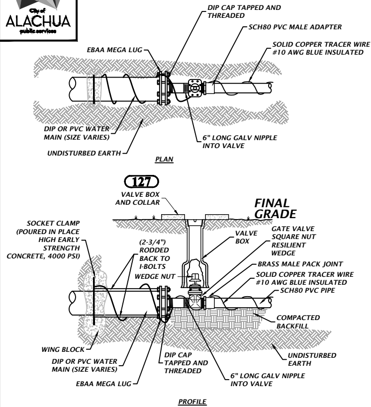
124 WATER MAIN REDUCTION OF LINE SIZE NTS
