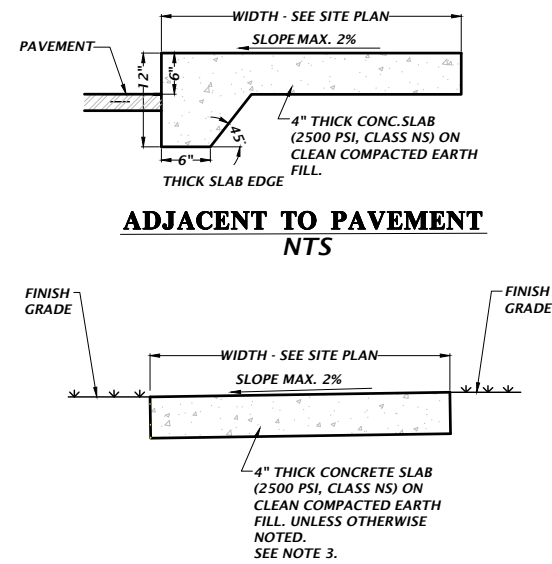
NOT ADJACENT TO PAVEMENT NTS
