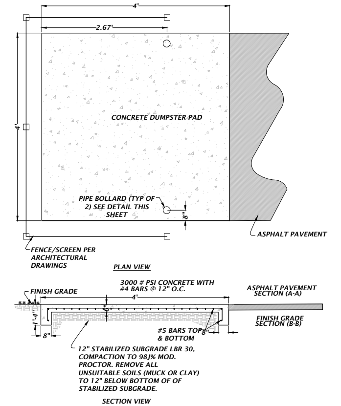
CONCRETE DUMPSTER PAD NTS
