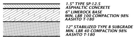
STANDARD DUTY ASPHALT, TYPE 2
