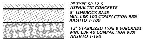
HEAVY DUTY ASPHALT
