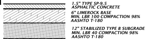
STANDARD DUTY ASPHALT, TYPE 1
