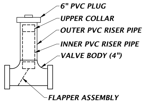
CLEAN CHECK BACKWASH VALVE NTS
