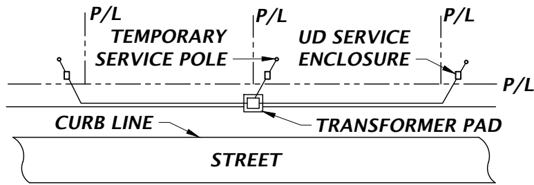
PLAN VIEW SHOWING TYPICAL PLACEMENT AT TEMPORARY UNDERGROUND SERVICE
