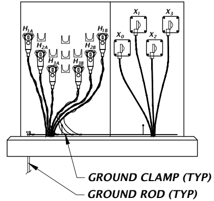
LOOP FEED FRONT ELEVATION, COVER REMOVED
