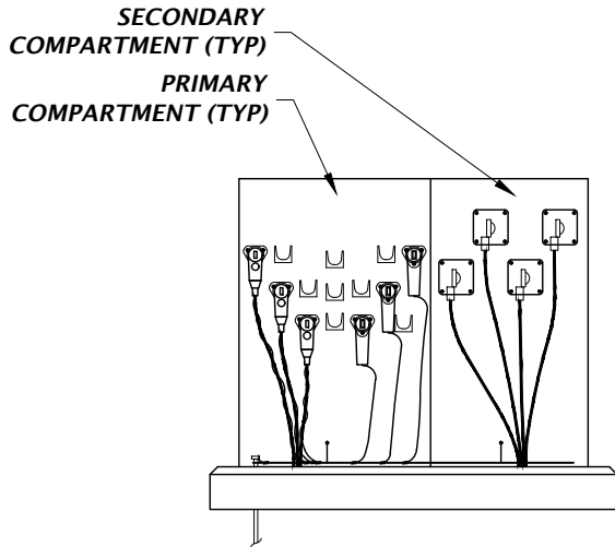
RADIAL FEED (LOOP TRANSFORMER) FRONT ELEVATION, COVER REMOVED
